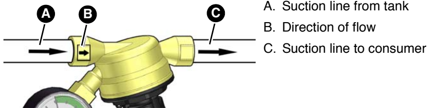
Fig. 4: Mounting
