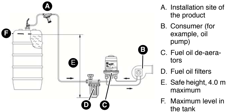
Fig. 6: Safe height = height difference between maximum level in the tank and lowest point of the supply line
